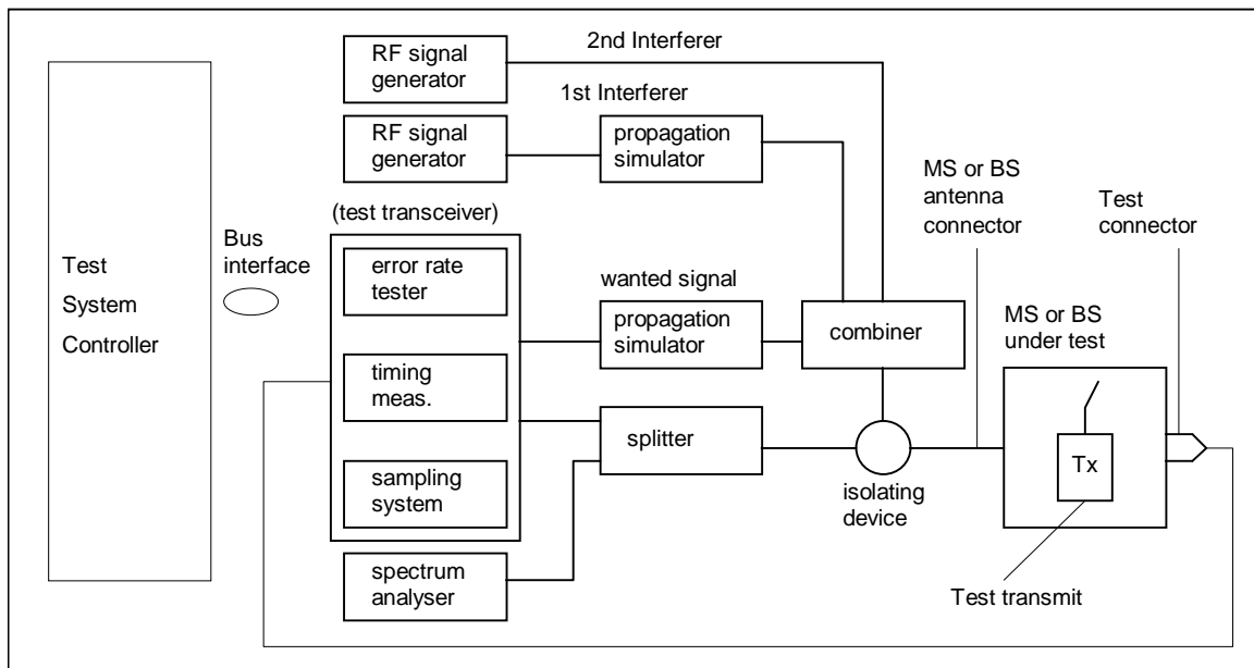
Figure 5.1: Radio test configuration
